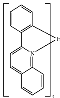
\text{Ir}(\text{2-phq})_3
