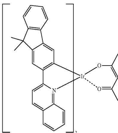
\text{Ir}(\text{flq})_2(\text{acac})
